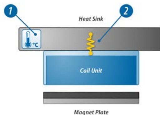
Picture 6 - Picture of the thermal resistance between coil unit and heat sink at a certain temperature.
