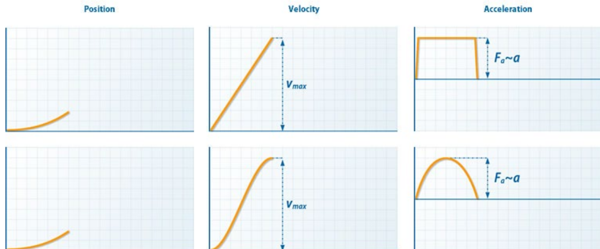
Picture 13 - Characteristics of a trapezoidal acceleration ramp defined by force (top) and a sinusoidal acceleration ramp defined by force (bottom).
