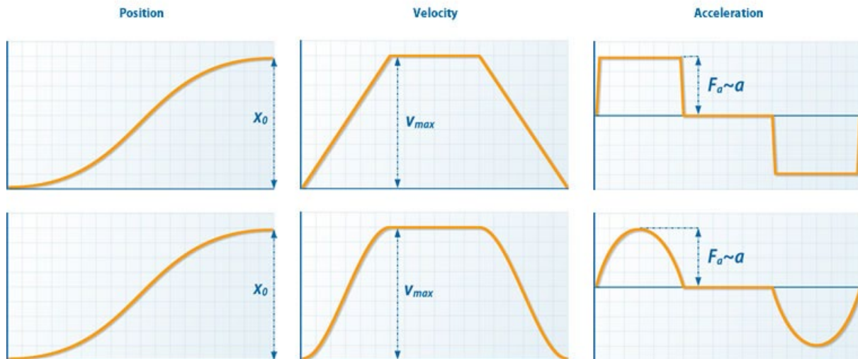
Picture 11 - Characteristics of a constant velocity trapezoidal movement profile (top) and a constant velocity sinusoidal movement (bottom).
