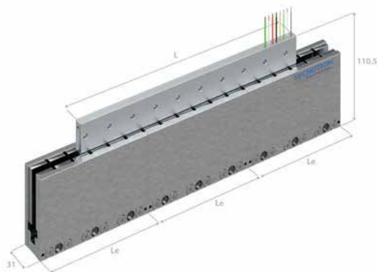
ULV9 G2 coil unit in 126mm magnet yokes
